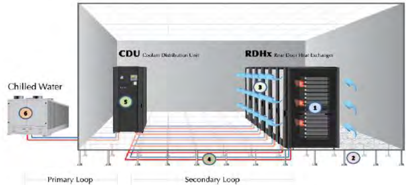
Figure 3. Coolcentric Rear Door Water Cooling System is Deployed on Each Rack
